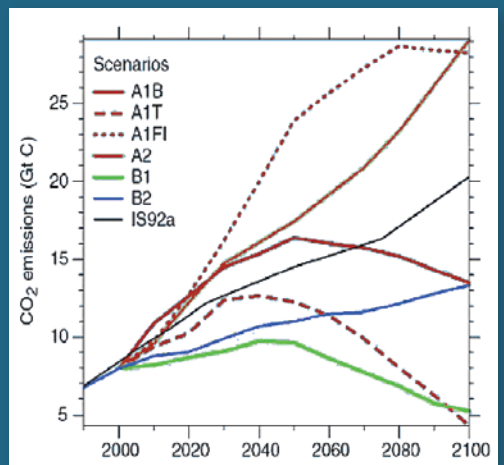
FIGURE 4-4 IPCC Future Scenarios
