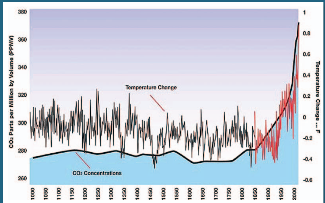
FIGURE 4-1 Concentrations of CO 2 (IPCC, 2007)
