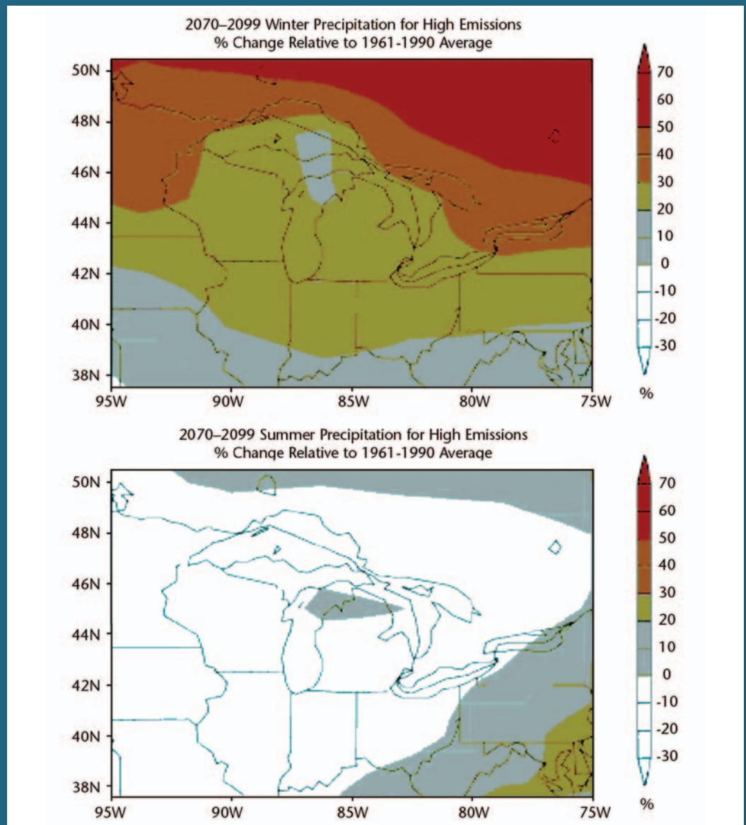
FIGURE 4-5 Midwest Shift in Seasonal Precipitation, Late 21st century
