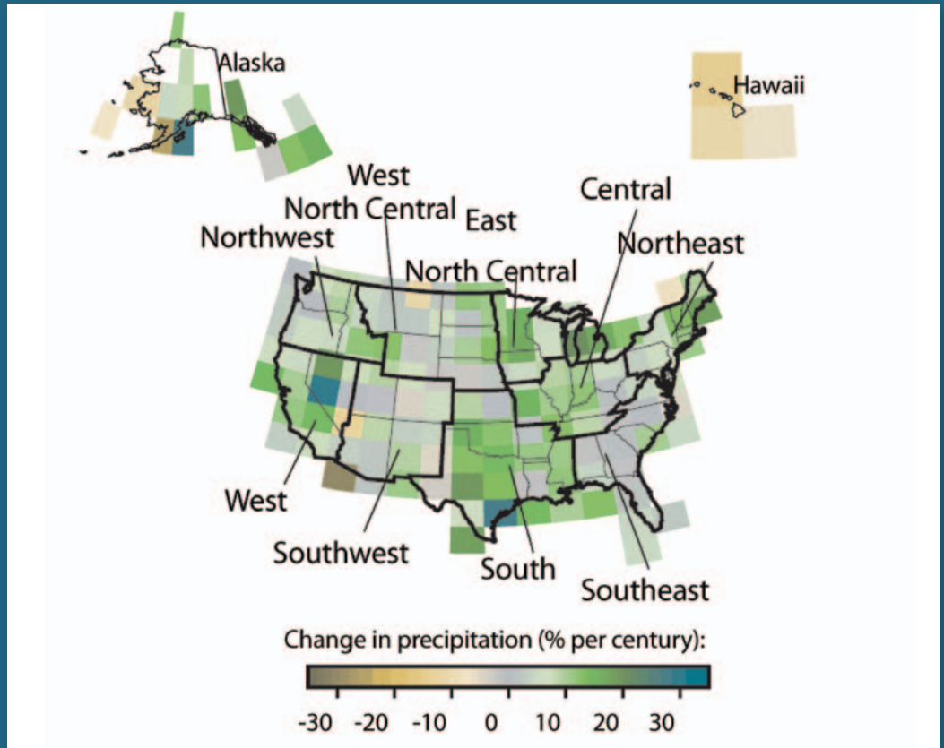
FIGURE 4-2 Average Precipitation Changes for the US
