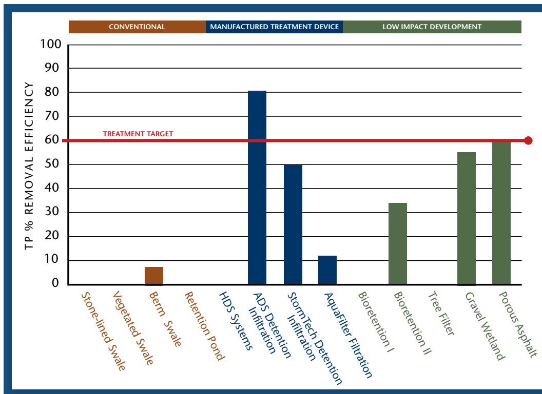
FIGURE 2-8 Phosphorus removal efficiencies for a range of stormwater BMPs; red line indicates commonly required performance treatment
