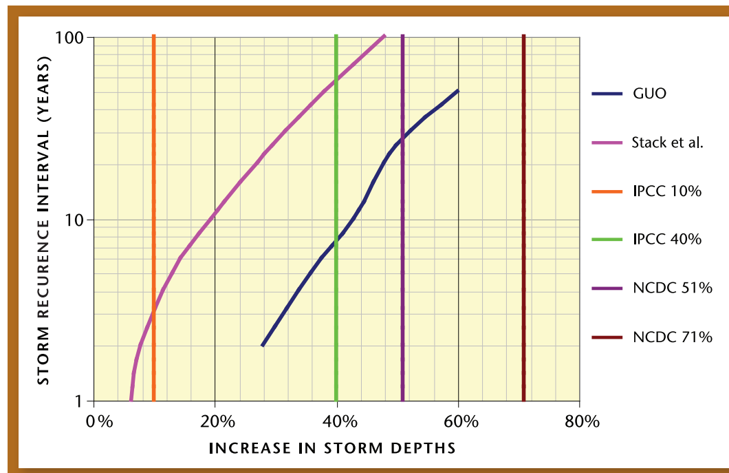
FIGURE 5-1 Changes in design storm depths predicted from different models of climate change
