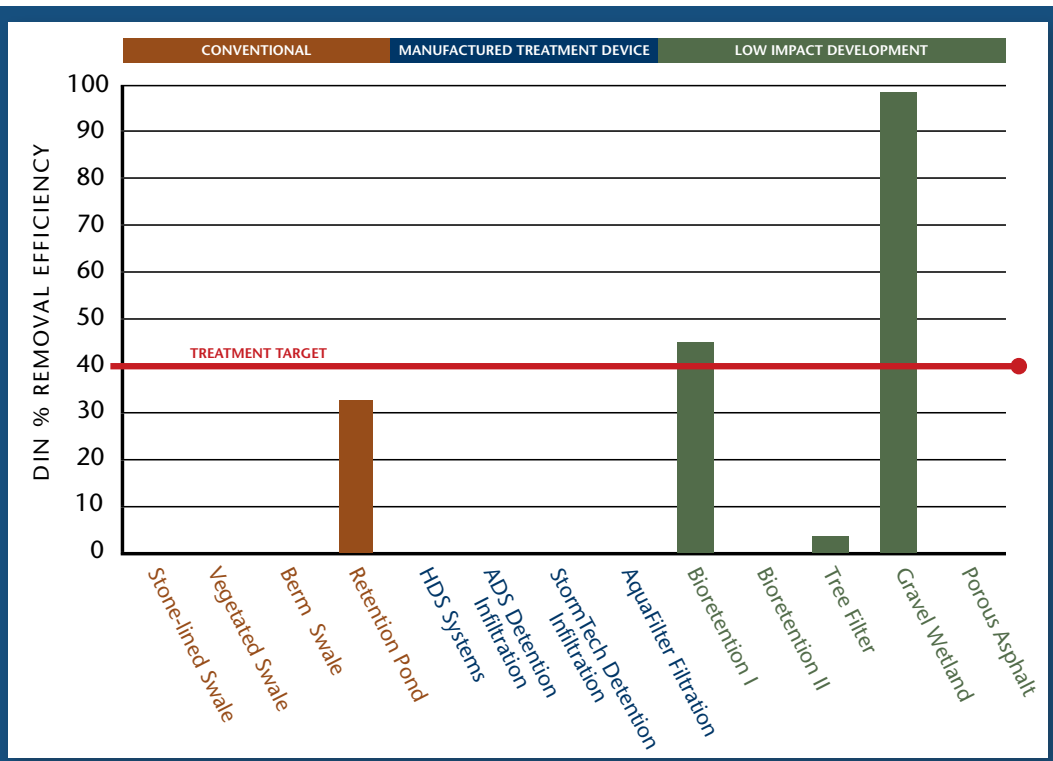
FIGURE 2-7 Nitrogen removal efficiencies for a range of stormwater BMPs; red line indicates commonly required performance treatment
