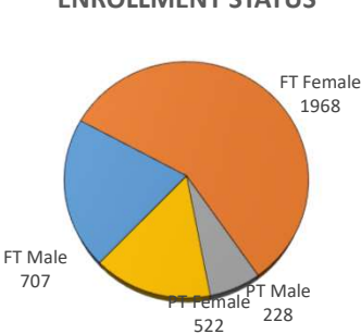
ENROLLMENT STATUS
