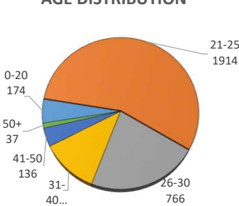
AGE DISTRIBUTION
