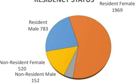
RESIDENCY STATUS
