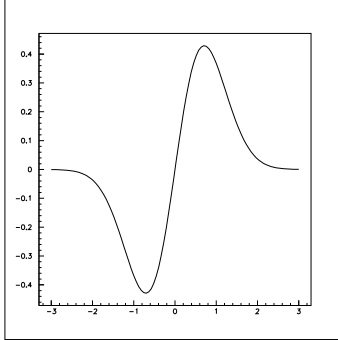
Figure 2: Energy Eigenstate
