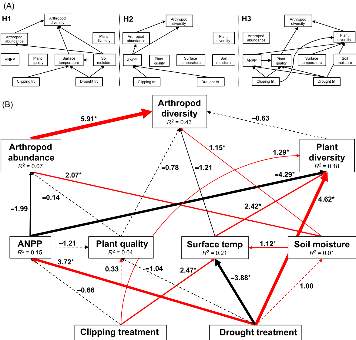
FIG. 1. Piecewise structural equation model (SEM) depicting the direct and indirect effects of drought and clipping on arthropod abundance and diversity. (A) Conceptual a priori models for each of the three hypotheses examined within our piecewise SEM (see Table 1 for hypotheses descriptions). (B) Piecewise SEM based on our a priori model. The piecewise SEM fit our data well: Fisher's C = 31.58 , AIC_c = 141.84 , P = 0.207 . Partial R^2 values are under each predicted variable, and standardized path estimates are provided next to each path with line thickness scaled based on the magnitude of the estimate (see Methods for variable descriptions). Red and black arrows indicate positive and negative relationships, respectively. Dashed arrows represent nonsignificant paths ( P > 0.05 ). Asterisks (*) indicate significance ( P < 0.05 ). Model estimates, standard errors, and P values are provided in Appendix S1: Table S2.
