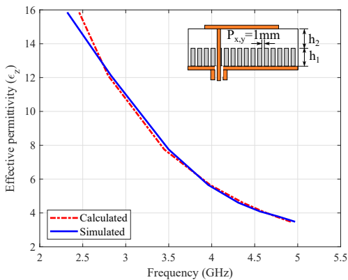
FIGURE 5: Effective permittivity ( \epsilon_z ) vs. resonant frequency of AADL MS patch antenna ( L = W = 14.7 mm) with different cylinder's height, diameter a = 0.5 mm and distance ( P_{x,y} ) of 1 mm between them in a dielectric host \epsilon_r = 3.48 .
