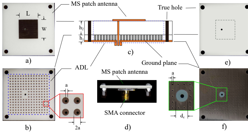
FIGURE 10: Prototype of the proposed AADL based frequency agile MS square patch antenna a) Top layer b) Bottom layer with AADL geometry. c) Side view of the proposed AADL based patch model. d) Side view of the AADL with an SMA connector. e) Bottom layer of top sub-dielectric. f) Bottom layer of bottom sub-dielectric. (Dimensions: L = W = 14.7 mm, a = 0.5 mm and dc = 4.25 mm)
