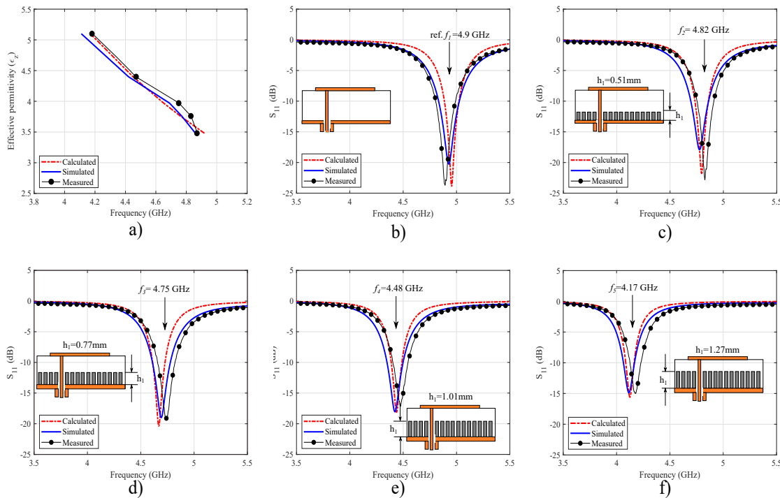
FIGURE 11: Calculated, simulated, and measured results of the proposed AADL MS square patch antenna a) Frequency vs. effective permittivity ( \epsilon_e ) b) Reference c) h_1 = 0.51 mm, h_2 = 1.52 mm d) h_1 = 0.77 mm, h_2 = 1.27 mm e) h_1 = 1.01 mm, h_2 = 1.01 mm f) h_1 = 1.27 mm, h_2 = 0.77 mm
