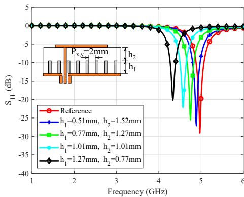
FIGURE 8: Simulated s -parameters vs. resonant frequency of AADL MS patch antenna ( L = W = 14.7 mm) with different cylinder's height, diameter a = 0.5 mm and distance ( P_{x,y} ) of 2 mm between them in a dielectric host \epsilon_r = 3.48 .
