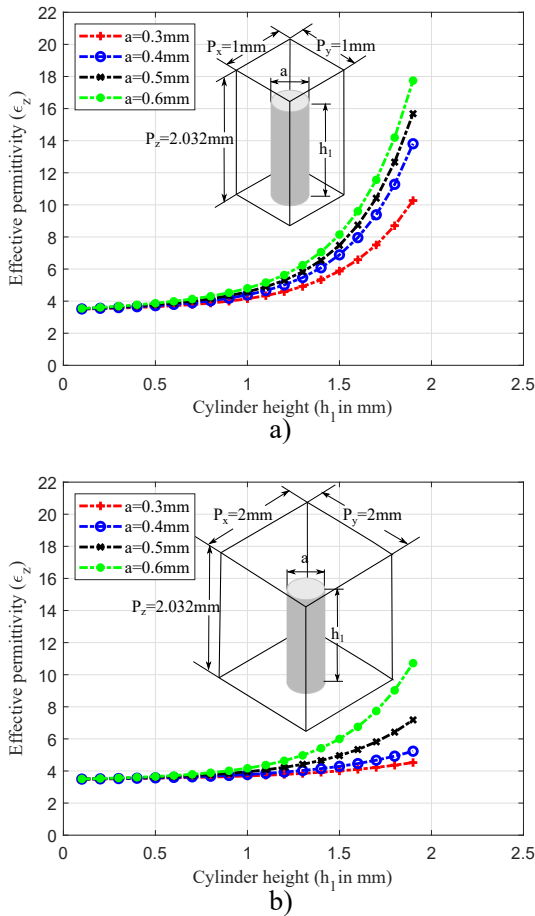
FIGURE 4: Calculated effective permittivity ( \epsilon_z ) vs. cylinder's height using a dielectric host of \epsilon_r = 3.48 for different diameters ( a = 0.3 mm to 0.6 mm). a) P_{x,y} = 1 mm. b) P_{x,y} = 2 mm.
