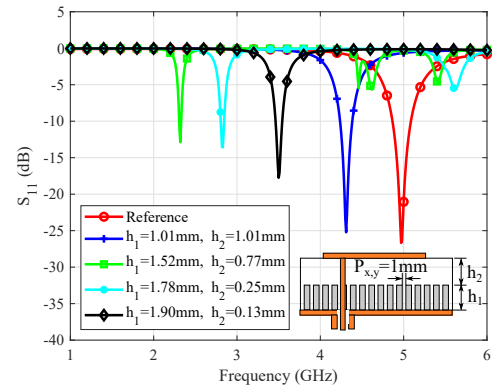
FIGURE 6: Simulated s -parameters vs. resonant frequency of AADL MS patch antenna ( L = W = 14.7 mm) with different cylinder's height, diameter a = 0.5 mm and distance ( P_{x,y} ) of 1 mm between them in a dielectric host \epsilon_r = 3.48 .
