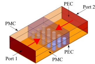
FIGURE 2: AADL geometry with PEC/PMC boundary conditions to extract \epsilon_z . s -parameters are obtained using embedding ports, indicated by arrows in red.
