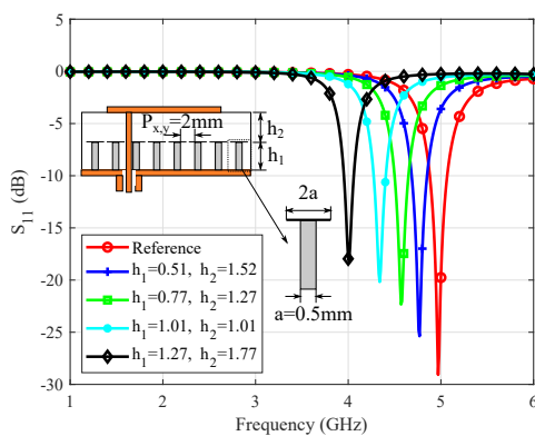
FIGURE 9: Simulated s -parameters of the AADL based MS square patch antenna ( L = W = 14.7 mm) after the inclusion of conducting rings onto the cylinders.
