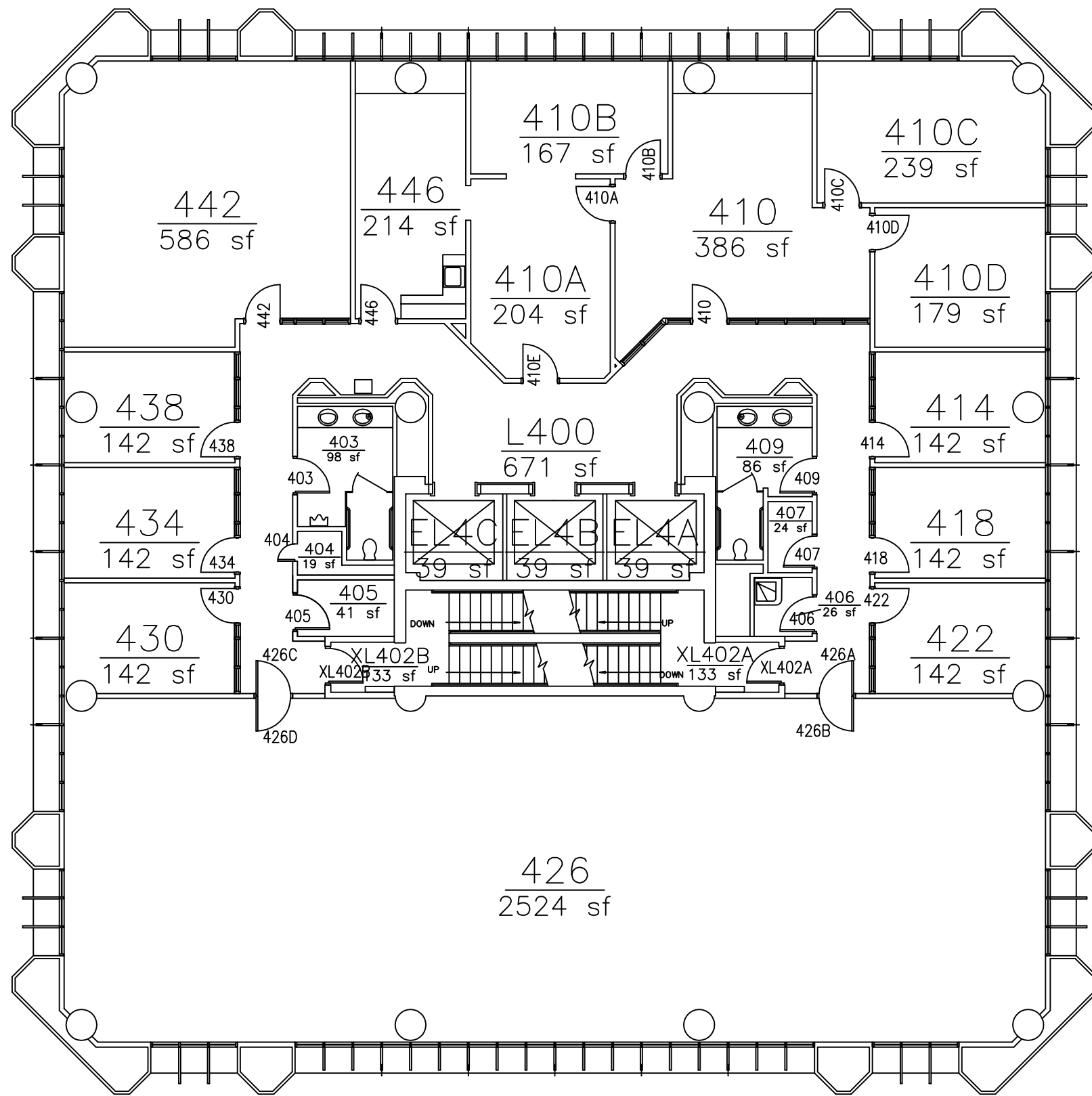
4 SARKEYS ENERGY CENTER TOWER - 4th FLOOR A4 NO SCALE
