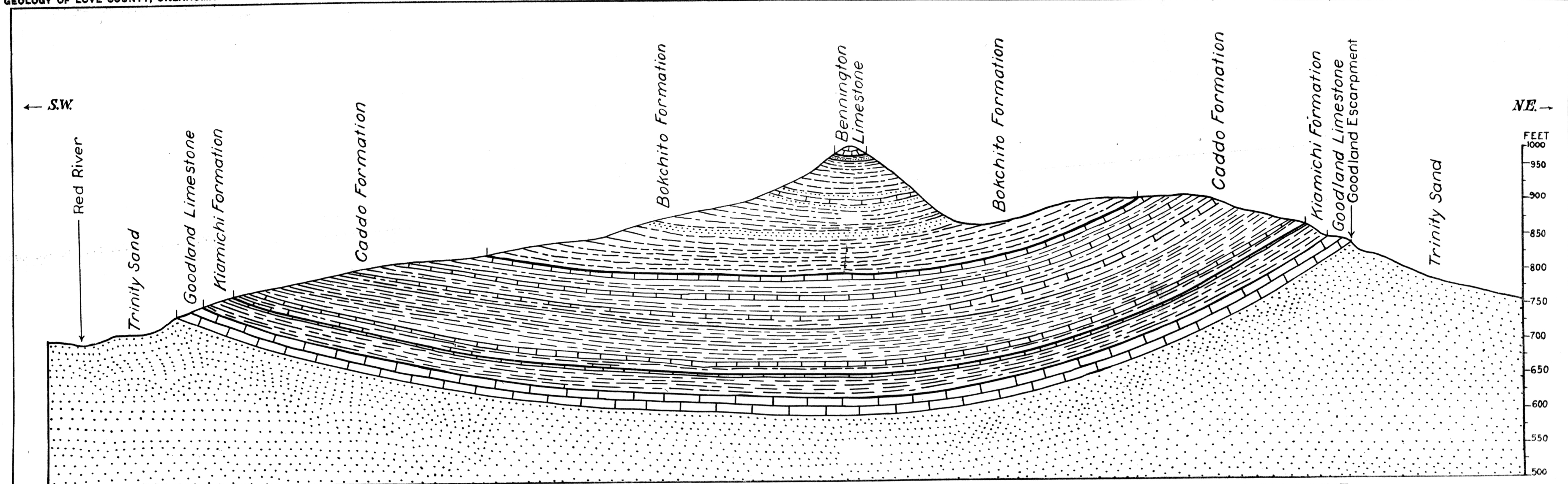
STRUCTURE SECTION (B-B' PL. XIX) SOUTHEAST OF MARIETTA, LOVE COUNTY, OKLA., ACROSS THE MARIETTA SYNCLINE
