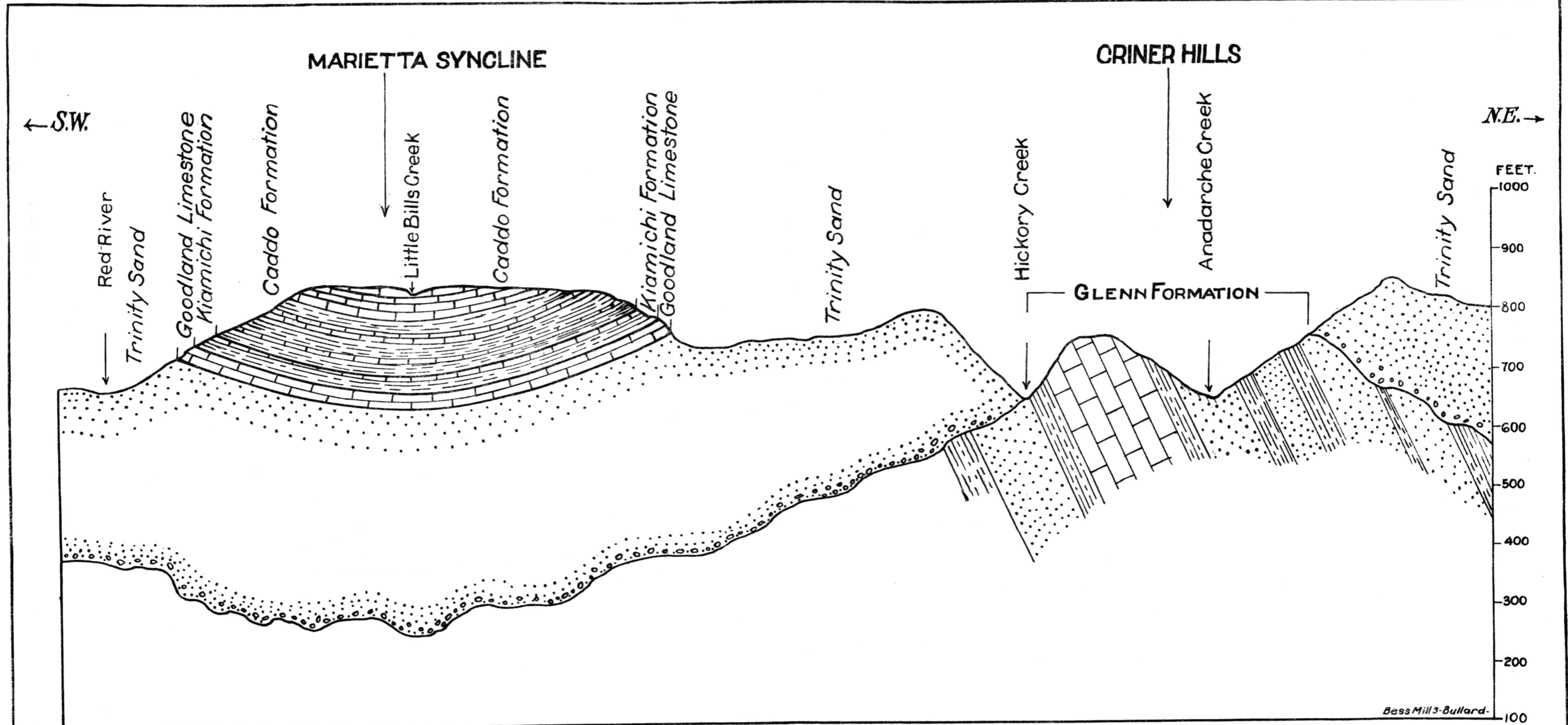
STRUCTURE SECTION (A-A' PIXIX) NORTHWEST OF MARIETTA, LOVE COUNTY, OKLA. SHOWING RELATION OF COMANCHEAN SEDIMENTS TO THE CRINER HILLS.
