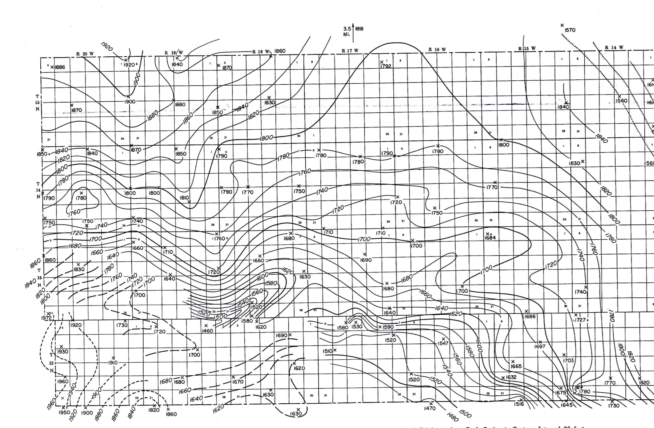
ISOPACH AND STRUCTURE CONTOUR MAPS OF PERMIAN RED BEDS, CUSTER COUNTY, OKLAHOMA ISOPACH CONTOUR INTERVAL 10 FEET, EXCEPT FOR RUSH SPRINGS; STRUCTURE CONTOUR INTERVAL 100 FEET, EXCEPT FOR SURFACE MAP
